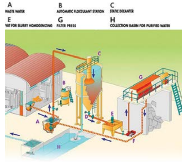
Water Treatment Plants by F&B Separates the waste product & water; recycled water returns for use. Systems eliminate sludge pits/monthly cleaning.
